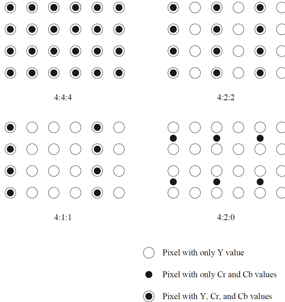
Fig. 5.6: Chroma subsampling
